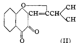
(II) Isopropylfurano-1,2-naphthoquinone
